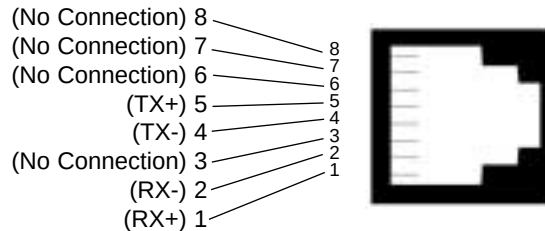
Figure 7: G.703/G.704 170 Ohm Connection.
