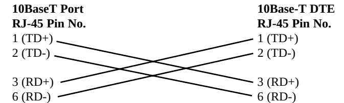
Figure 8: 10Base-T Cross-over Cable Connection
