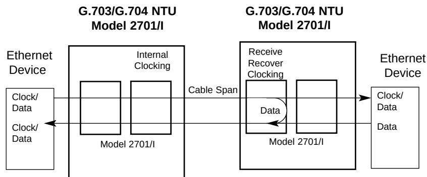
Figure 13. Remote Loop in a Network Extension Application
