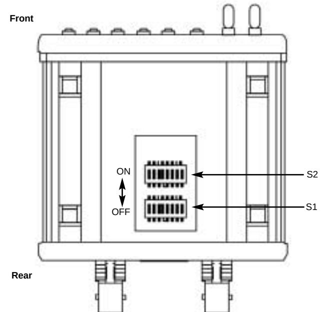
Figure 3. Underside of Model 2701/I, Showing Location of DIP Switches
