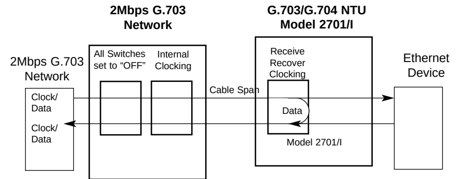
Figure 12. Local Loopback for a Network Termination Application
