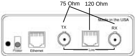
Figure 5. Model 2701/I Rear Panel
