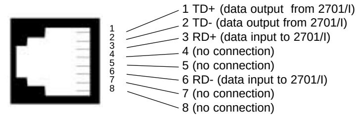
Figure 8: Connecting the 10Base-T Ethernet Port to a PC
