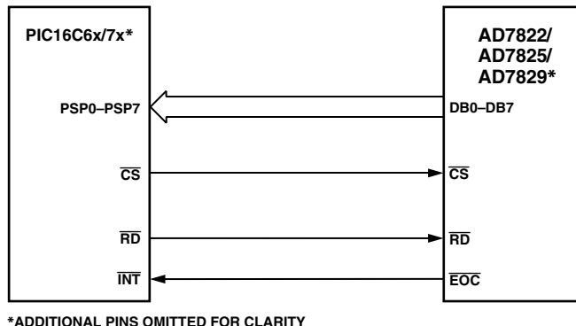
Figure 24. Interfacing to the PIC16C6x/7x
