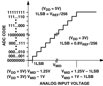
Figure 6. Transfer Characteristic
