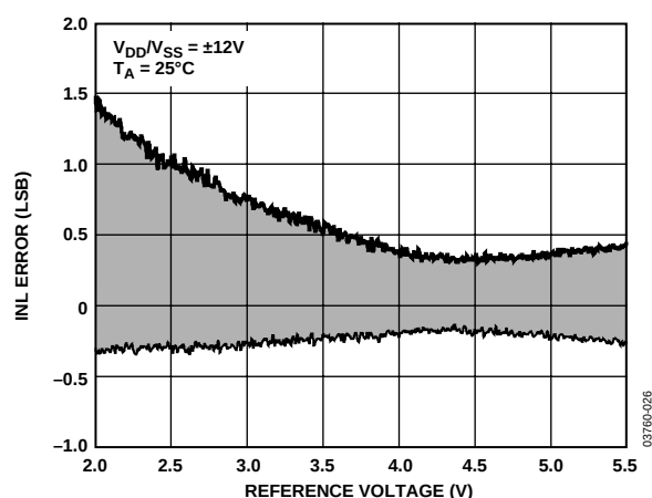
Figure 17. Integral Nonlinearity Error vs. Reference Voltage, ±12 V Supplies
