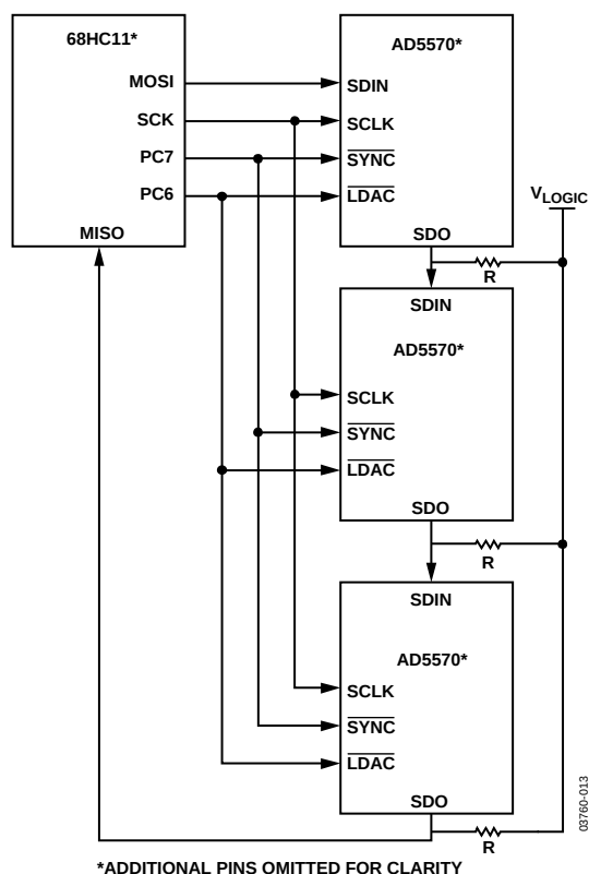
Figure 38. Daisy Chaining Using the AD5570
