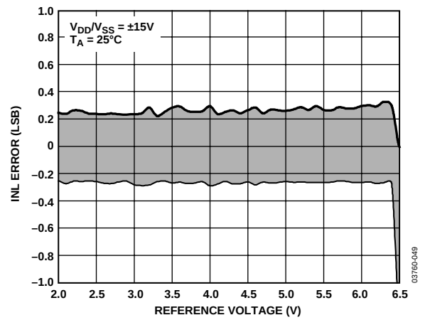
Figure 21. Differential Nonlinearity Error vs. Reference Voltage, \pm 15 V Supplies
