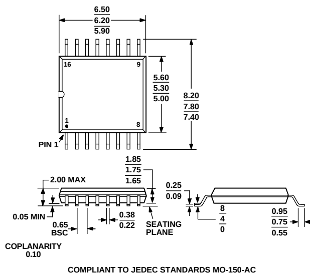
Figure 47. 16-Lead Shrink Small Outline Package [SSOP] (RS-16) Dimensions shown in millimeters
