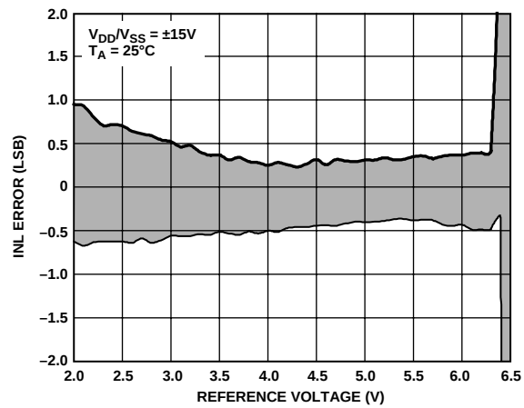
Figure 20. Integral Nonlinearity Error vs. Reference Voltage, \pm 15 V Supplies
