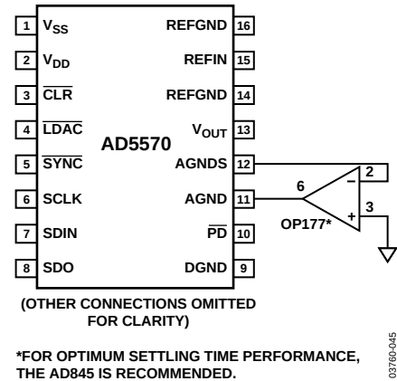
Figure 40. Driving AGND and AGNDS Using a Force/Sense Amplifier
