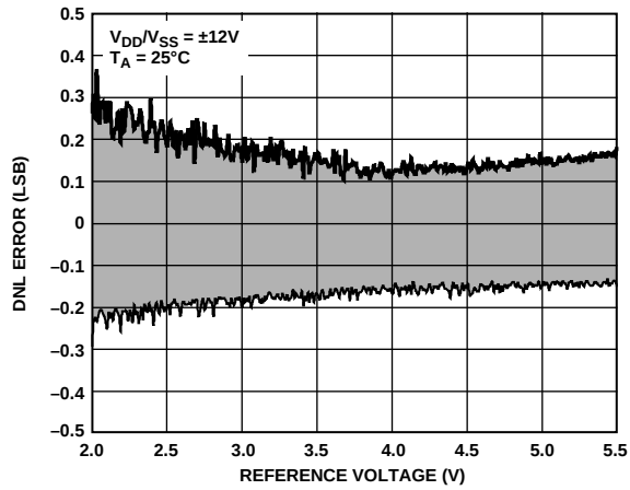
Figure 18. Differential Nonlinearity Error vs. Reference Voltage, \pm 12 V Supplies
