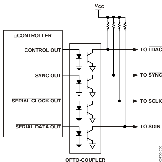
Figure 41. Opto-Isolated Interface
