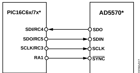
Figure 45. AD5570 to PIC16C6x/7x Interface
