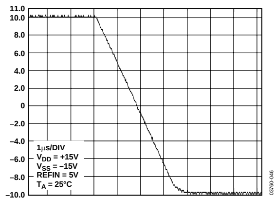
Figure 28. Settling Time
