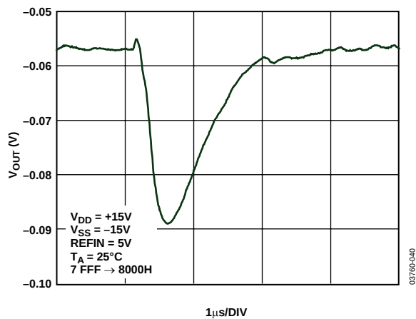
Figure 32. Major Code Transition Glitch Energy, \pm 15\text{V} Supplies
