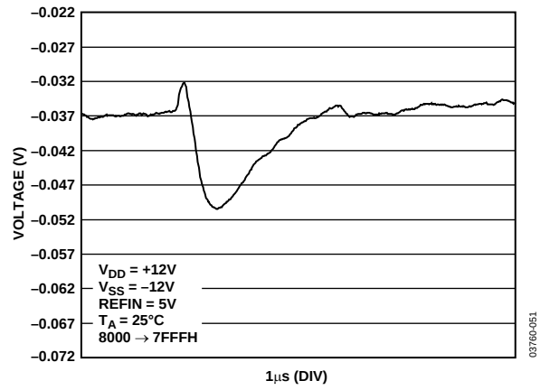
Figure 33. Major Code Transition Glitch Energy, \pm 12\text{V} Supplies
