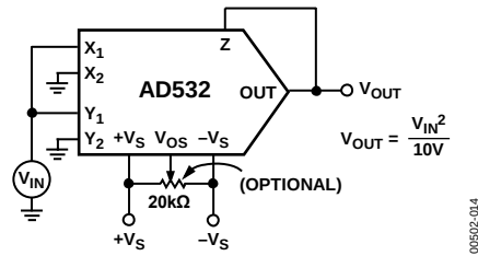
Figure 16. Squarer Connection
