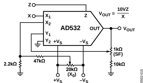
Figure 17. Divider Connection
