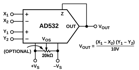
Figure 15. Multiplier Connection
