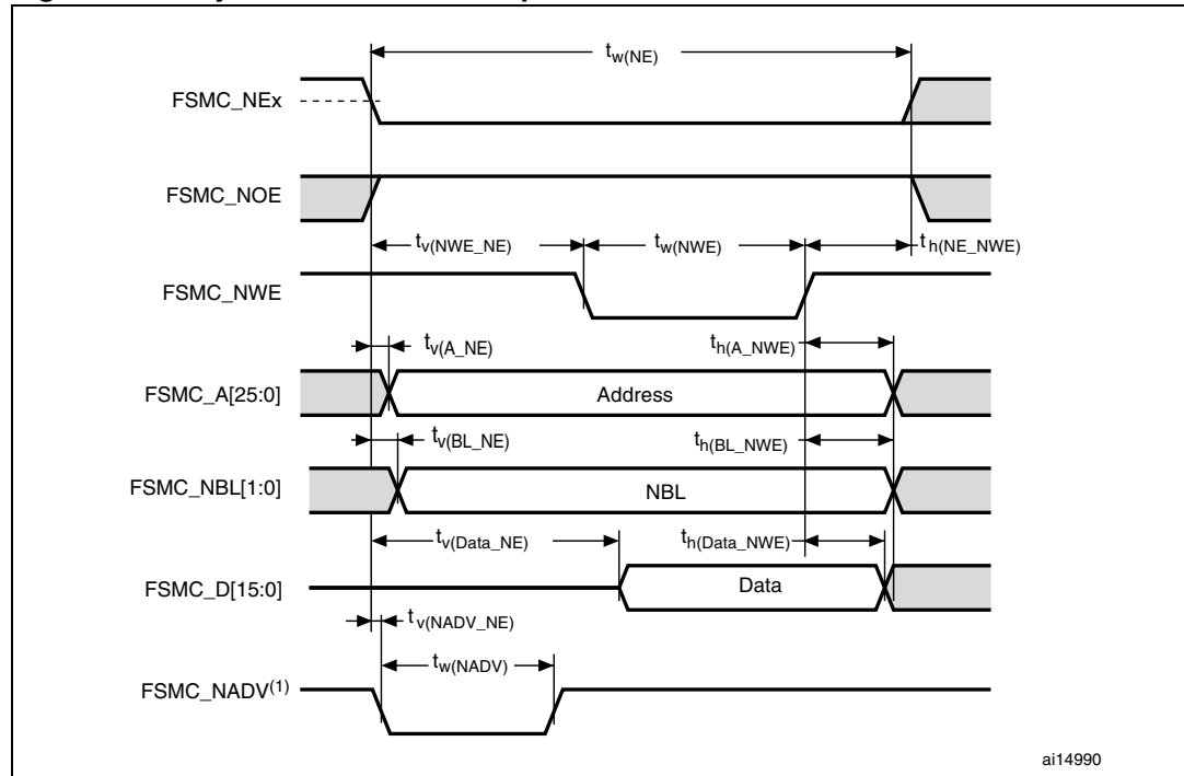
Figure 22. Asynchronous non-multiplexed SRAM/PSRAM/NOR write waveforms
