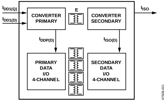
Figure 16. Power Consumption Within the ADuM5400
