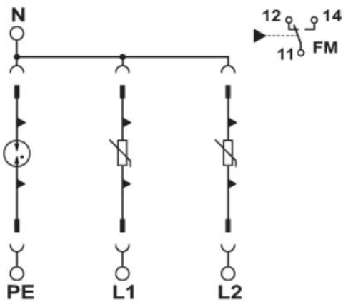
Circuit diagram
