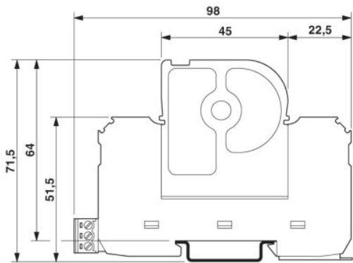
Dimensioned drawing
