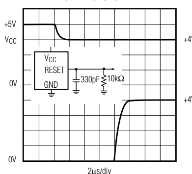
MAX813L RESET RESPONSE TIME
