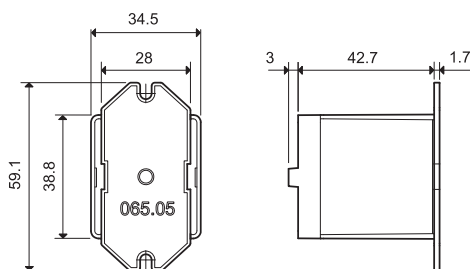
Top flange mount for types 65.31.xxxx.xxx9
