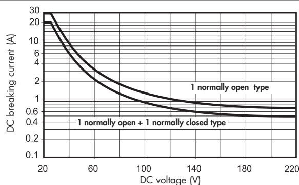
H 65 - Maximum DC1 breaking capacity
