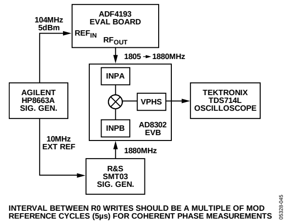
Figure 19. Test Setup for Phase Lock Time Measurement
