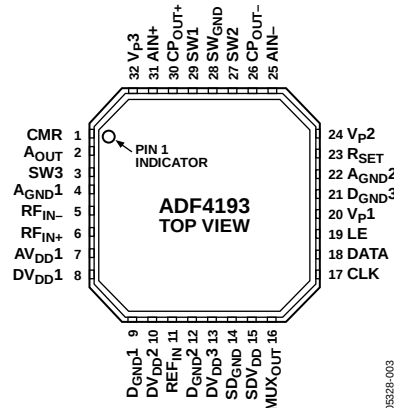
Figure 3. Pin Configuration
