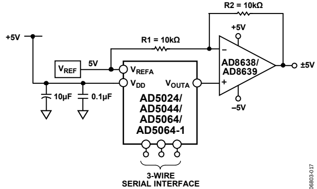
Figure 57. Bipolar Operation
