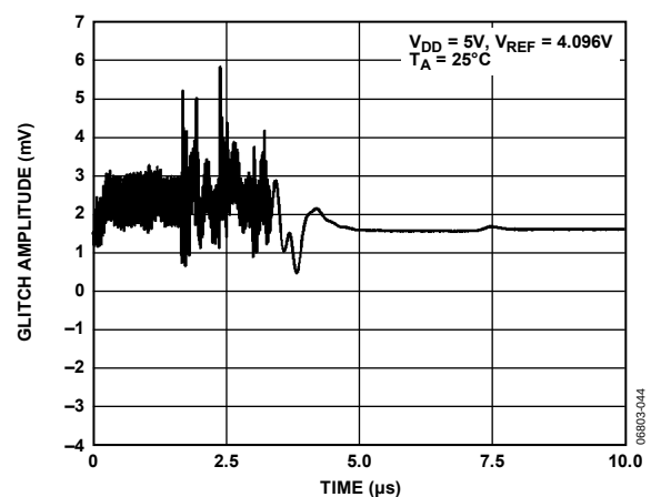
Figure 33. DAC-to-DAC Crosstalk
