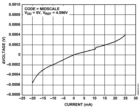
Figure 40. Typical Output Load Regulation
