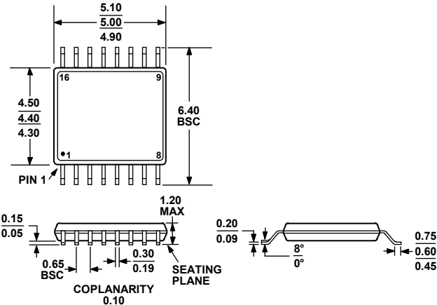
COMPLIANT TO JEDEC STANDARDS MO-153-AB Figure 60. 16-Lead Thin Shrink Small Outline Package [TSSOP] (RU-16) Dimensions shown in millimeters
