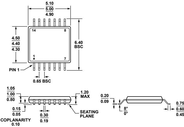
COMPLIANT TO JEDEC STANDARDS MO-153-AB-1 Figure 59. 14-Lead Thin Shrink Small Outline Package [TSSOP] (RU-14) Dimensions shown in millimeters
