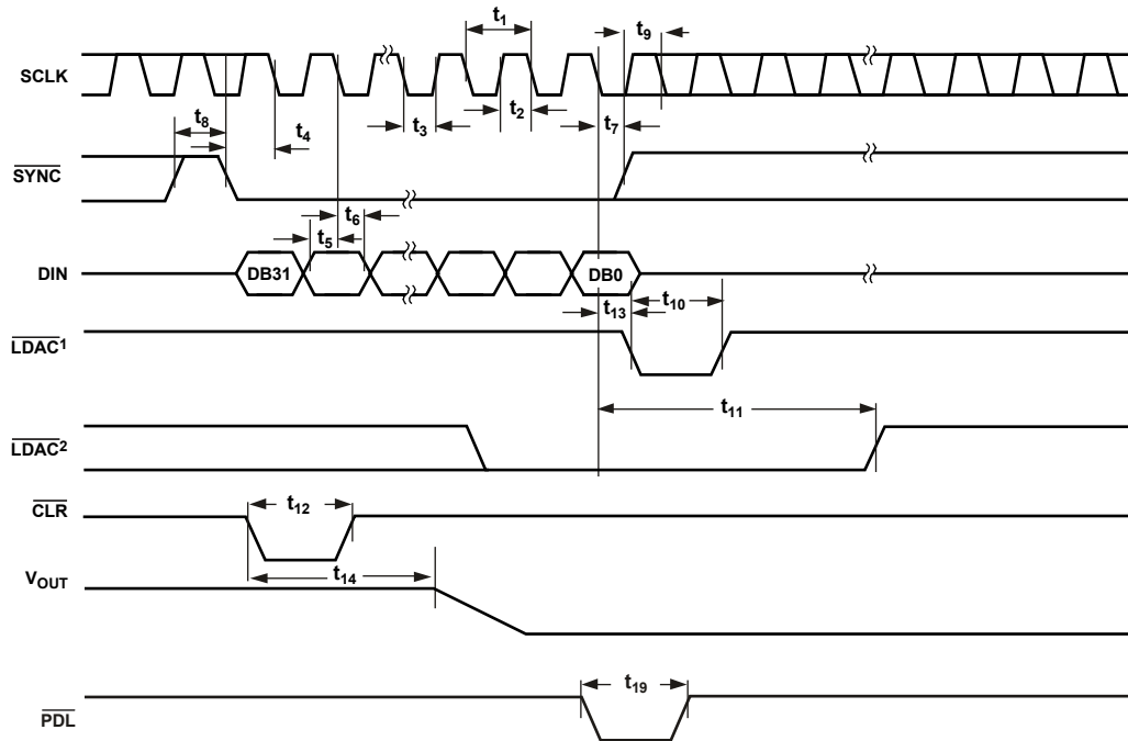
Figure 4. Serial Write Operation
