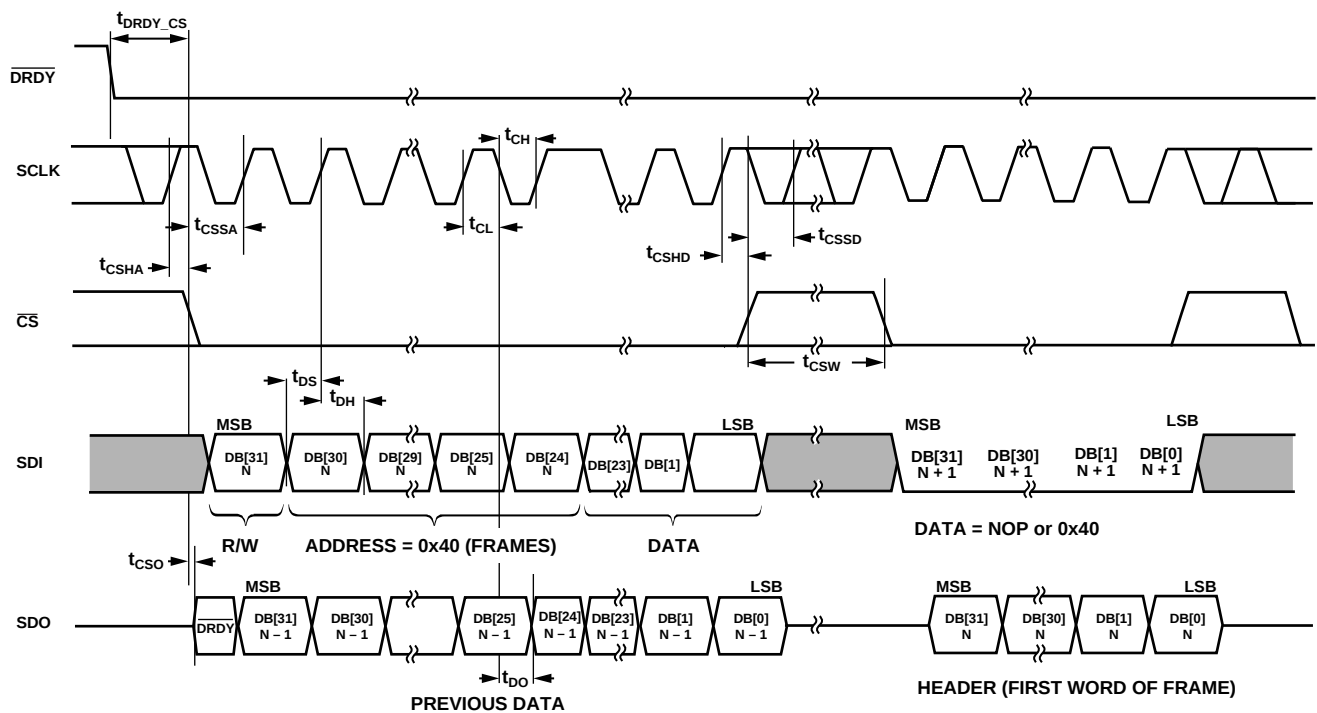
图3. 开始读取帧数据( \text{CPHA} = 1 , \text{CPOL} = 1 )
