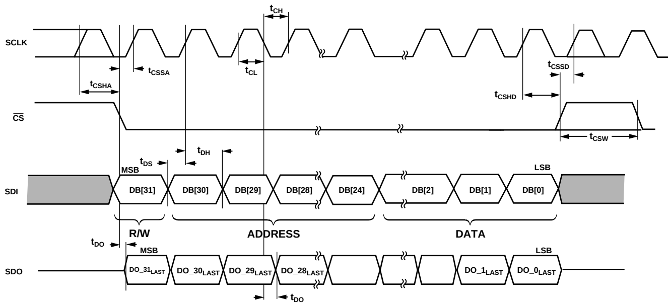
图4. 数据读取和写入时序图( \text{CPHA} = 0 , \text{CPOL} = 0 )
