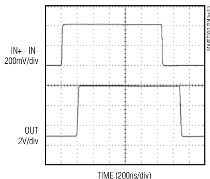
PROPAGATION DELAY
