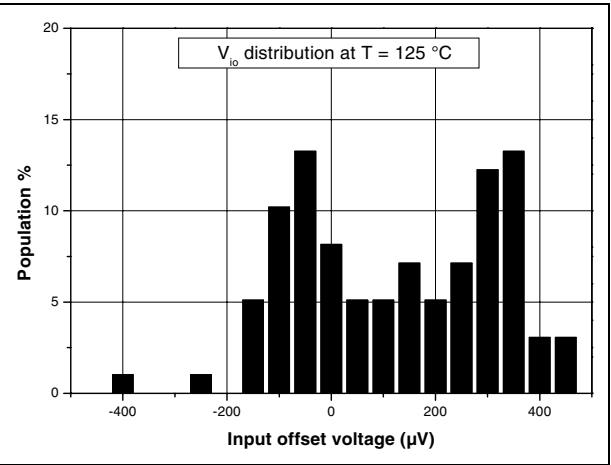
Figure 3. V_{io} distribution at V_{cc} = \pm 15\text{ V} and T = 125^\circ\text{C}
