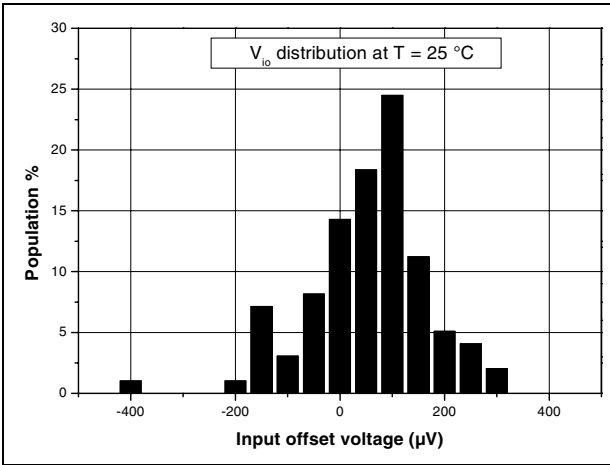
Figure 2. V_{io} distribution at V_{cc} = \pm 15\text{ V} and T = 25^\circ\text{C}
