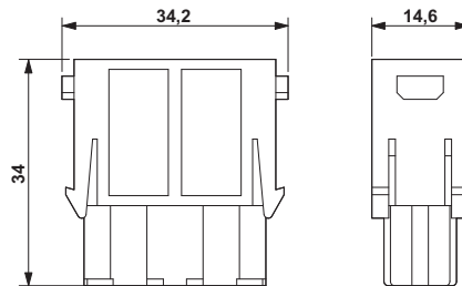
Female insert
