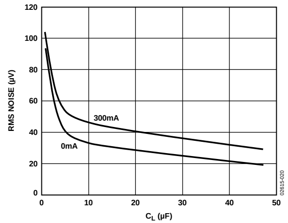
Figure 20. RMS Noise vs. C_L (10 Hz to 100 kHz)
