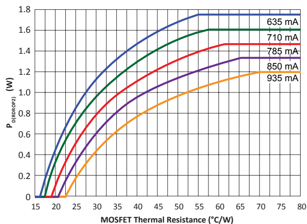
Figure 13. R_{\text{DROP1}} power dissipation versus 3.3 V MOSFET thermal resistance at various 3.3 V regulator maximum current settings
