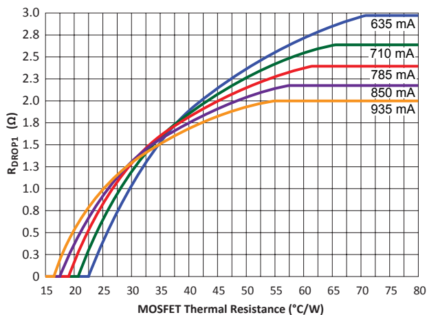
Figure 12. R_{\text{DROP1}} value versus 3.3 V MOSFET thermal resistance at various 3.3 V regulator maximum current settings
