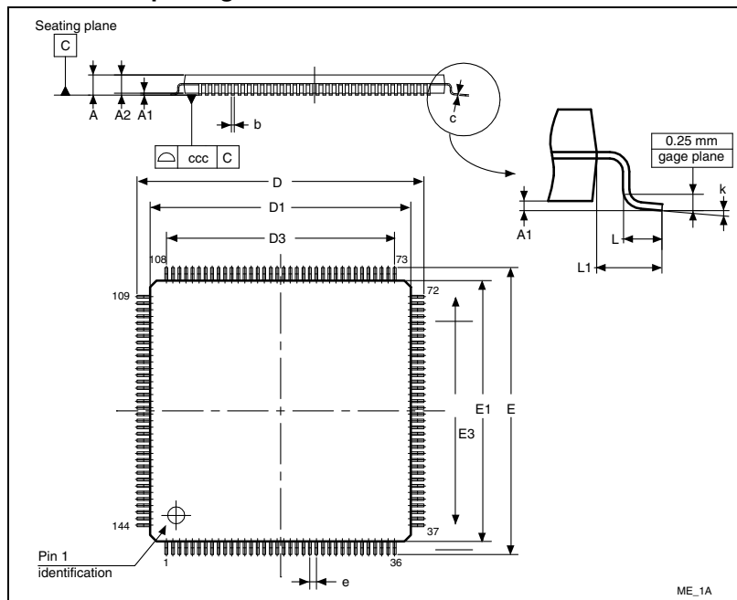
Figure 52. LQFP144, 20 x 20 mm, 144-pin thin quad flat package outline (1)
