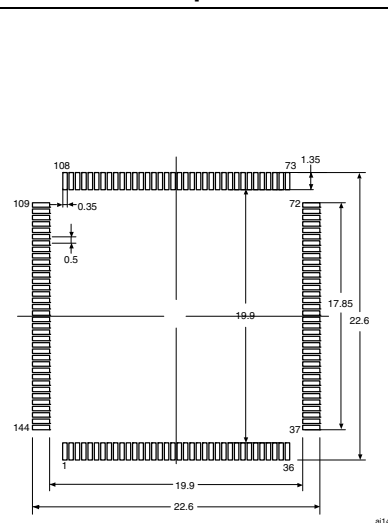
Figure 53. Recommended footprint (1)(2)
