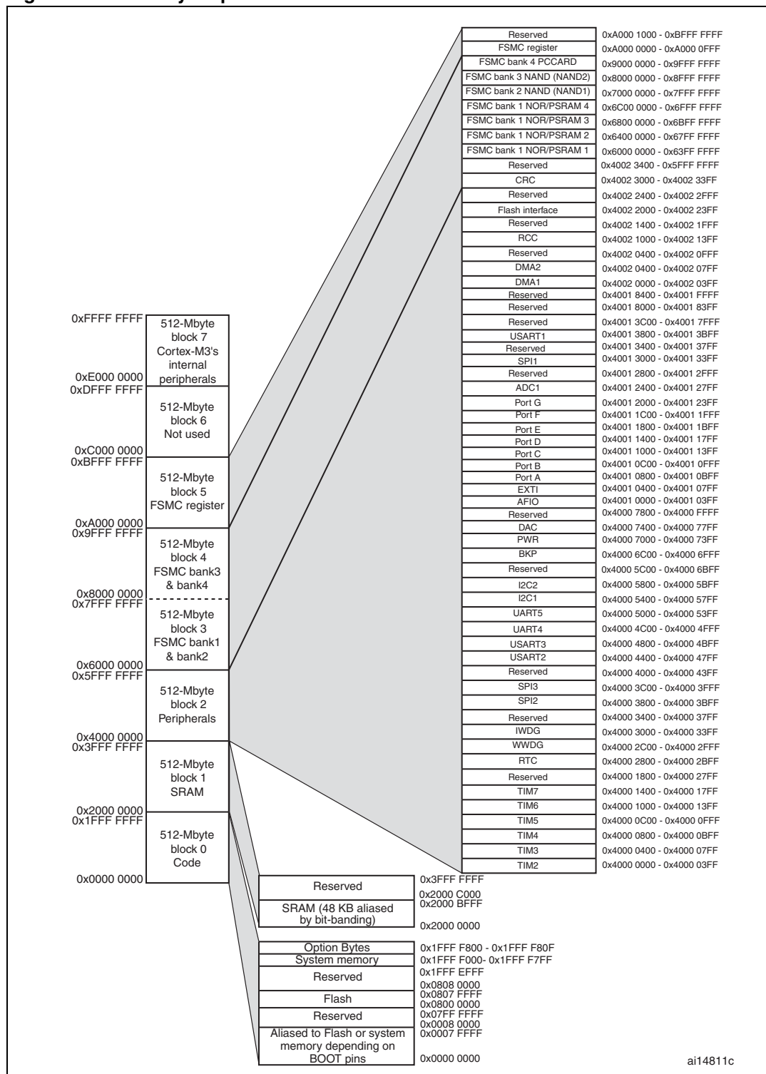
Figure 6. Memory map
