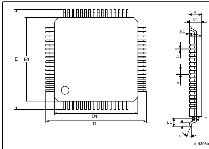
Figure 56. LQFP64 – 10 x 10 mm, 64 pin low-profile quad flat package outline (1)
