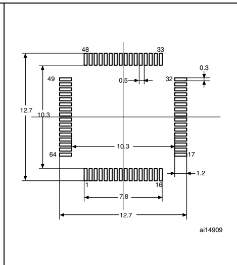
Figure 57. Recommended footprint (1)(2)
