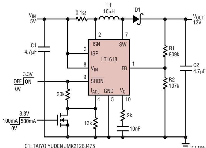
USB to 12V Boost Converter (with Selectable 100mA/500mA Input Current Limit)
