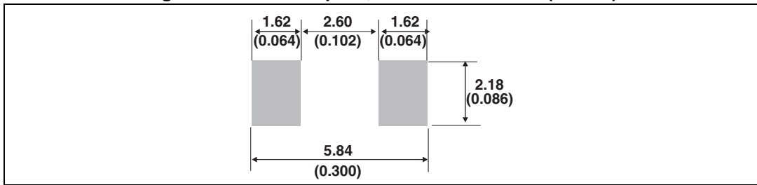
Figure 22. SMB marking layout
