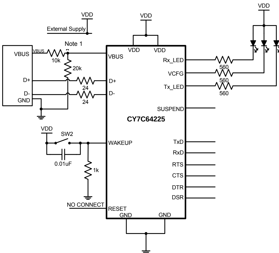
Figure 5. Self Powered Design (VDD = 3.3 V)
