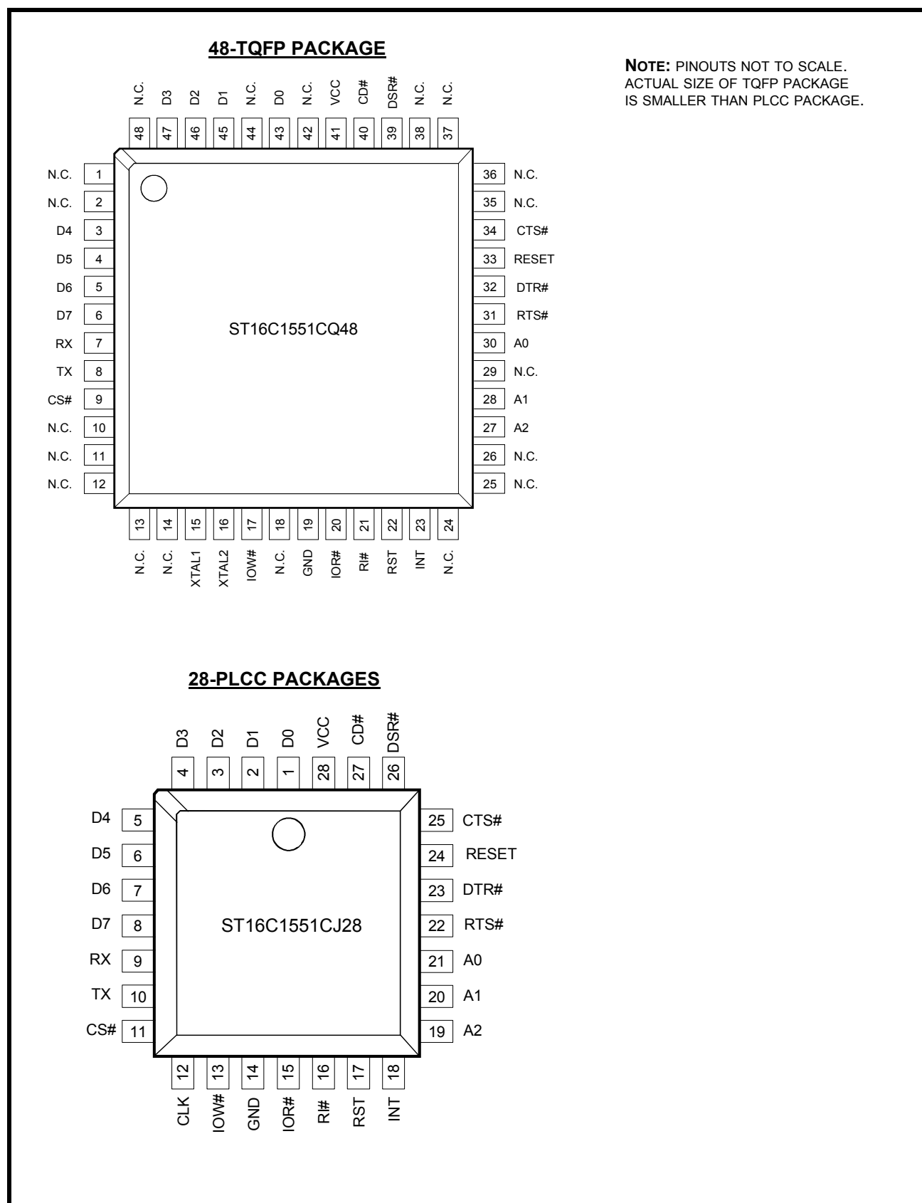
FIGURE 3. ST16C1551 PINOUTS
