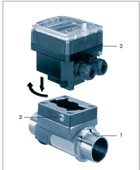
Fig. 3.2 Mounting 8035
