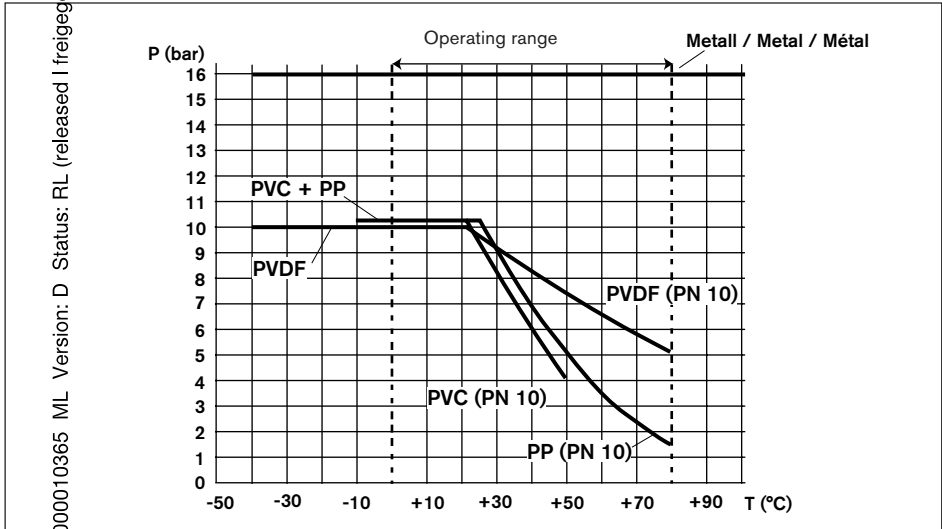
Fig. 3.1 Temperature-pressure dependence
