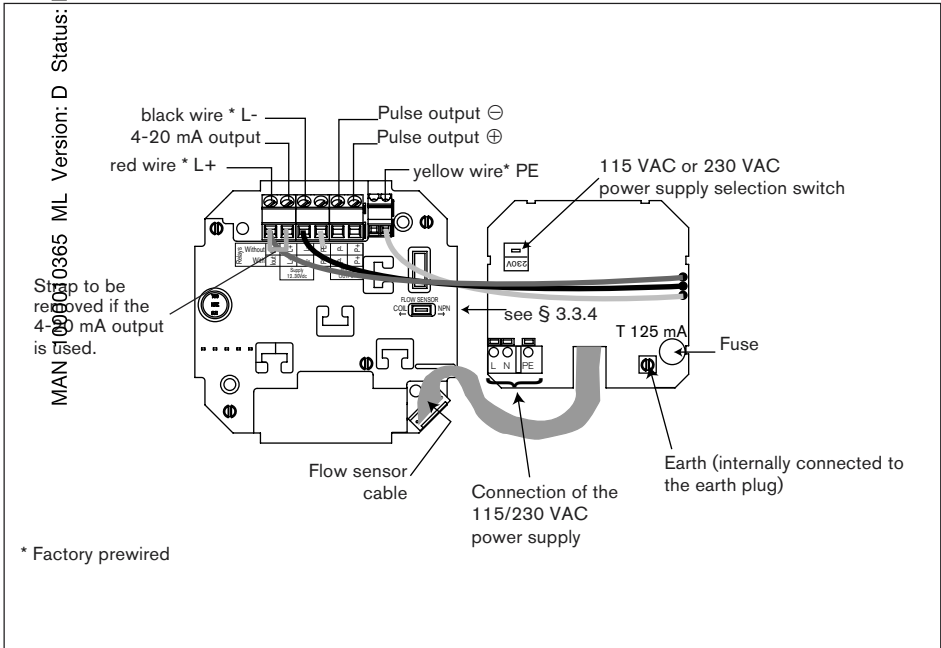
Fig. 3.10 Wiring of the SE35, 115/230 VAC, without relay, with cable glands
