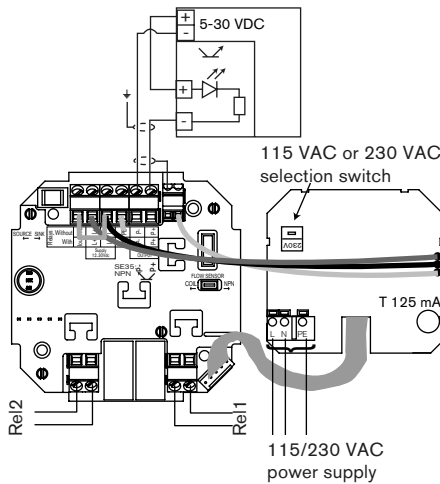
Fig. 3.13 Connection of electronic module SE35, 115/230 VAC, with relays and cable glands, to a PLC.
