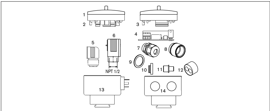
Fig. 5.1 Spare parts explosion drawing SE35
