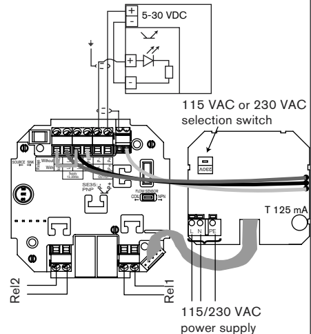
Fig. 3.13 Connection of electronic module SE35, 115/230 VAC, with relays and cable glands, to a PLC.
