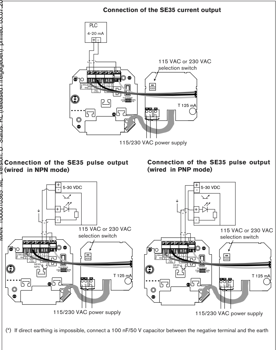
Fig. 3.11 Connection of electronic module SE35, 115/230 VAC, without relay, with cable glands, to a PLC.
