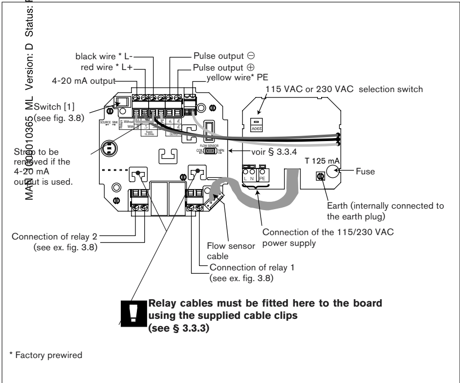
Fig. 3.12 Wiring of the SE35, 115/230 VAC, with relays and cable glands
