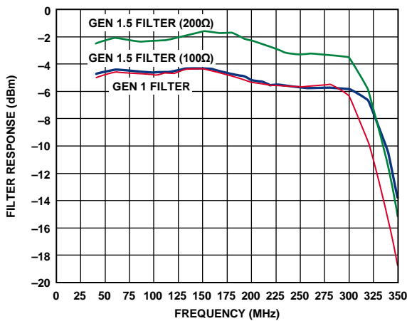
Figure 38. Frequency Response of the DAC + the Filter + the Modulator
