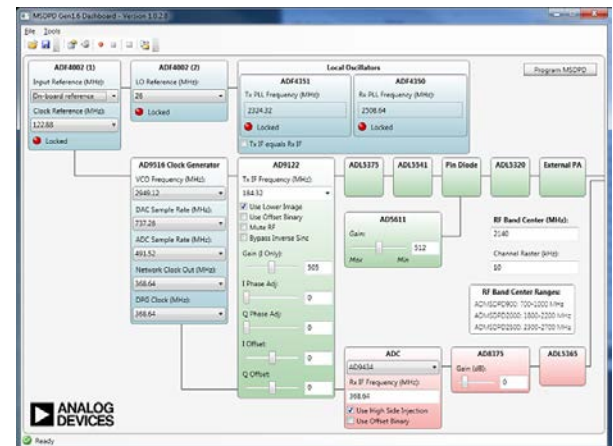
Figure 59. MSDPD Gen1.6 Dashboard
