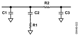
Figure 22. ADF4002 (1) Loop Filter Design
