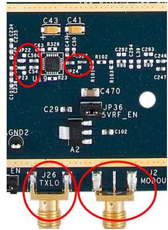
Figure 39. ADL5375 Placement
