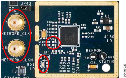
Figure 27. AD9516-0 Placement
