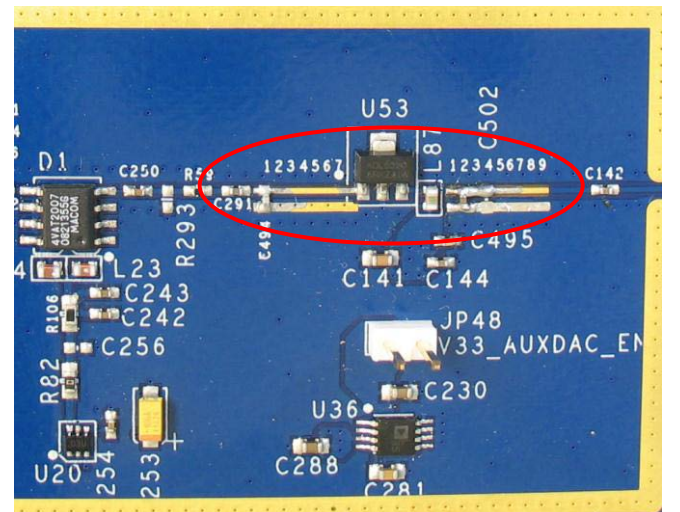
Figure 43. Location of ADL5320 Tuning Components
