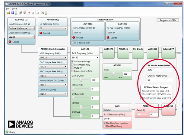
Figure 10. Select RF Band Center Frequency
