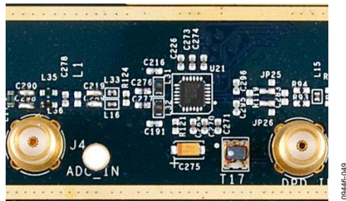
Figure 49. AD8375 Placement
