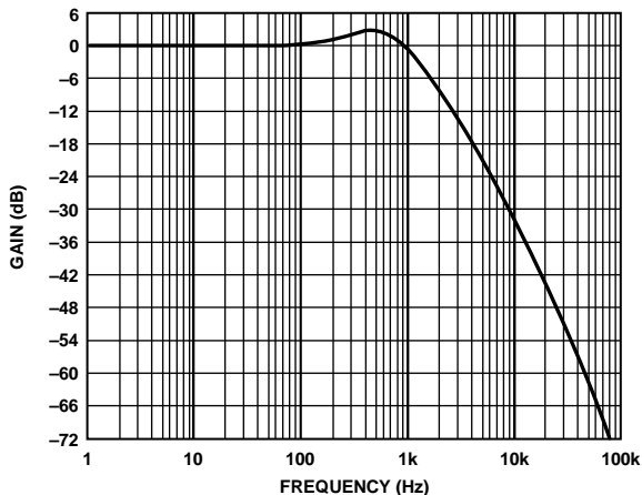
Figure 23. ADF4002 (1) Loop Filter Frequency Response
