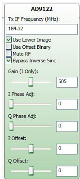
Figure 64. AD9122 Controls
