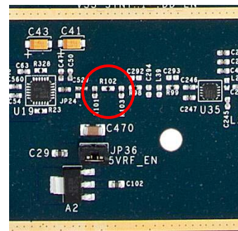
Figure 40. PI Attenuator
