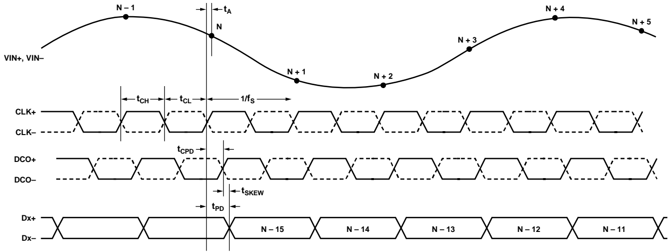
Figure 57. AD9434 Output Data Timing
