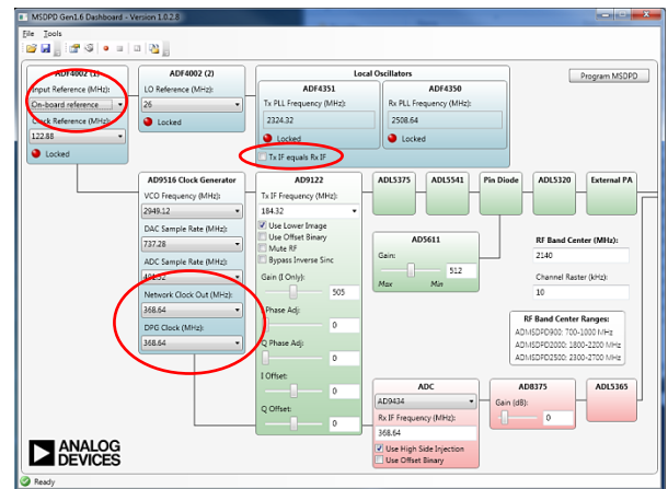
Figure 11. Clock Control
