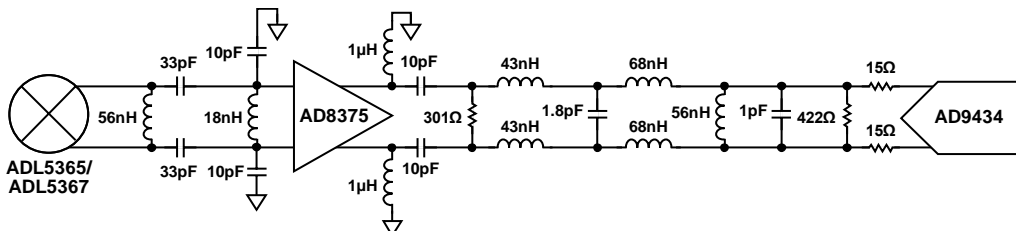
Figure 51. Antialiasing Filter Structure
