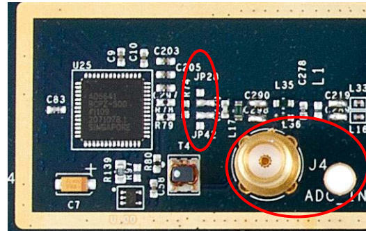
Figure 50. ADC Placement
