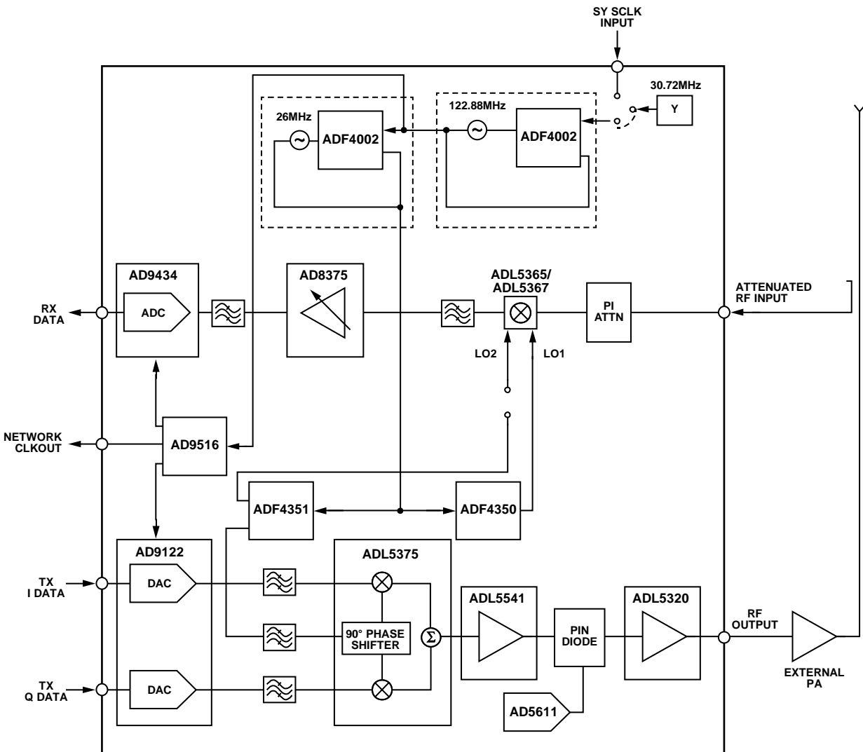
Figure 2. MSDPD Board Block Diagram
