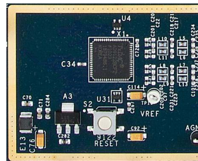
Figure 36. AD9122 Placement
