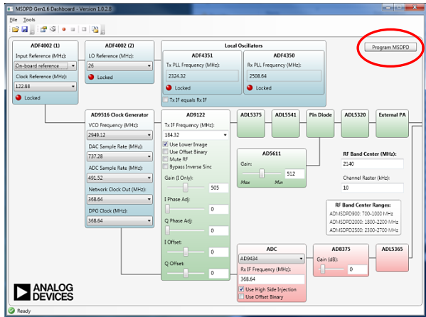
Figure 12. Program MSDPD
