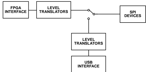
Figure 58. SPI Bridge Block Diagram
