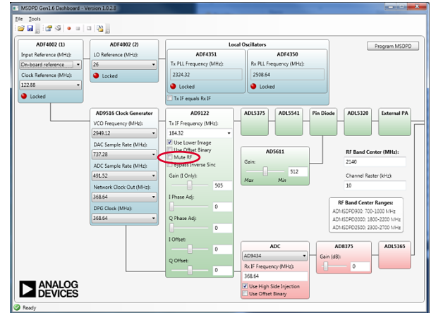
Figure 16. Mute RF
