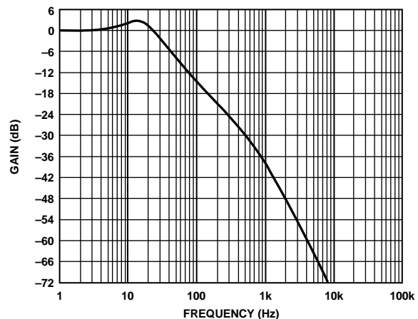
Figure 26. ADF4002 (2) Loop Filter Frequency Response
