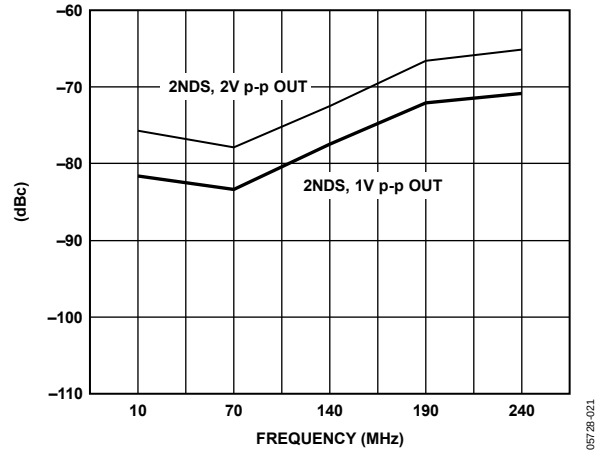
Figure 28. Single-Ended, Second-Order Harmonic Distortion, 200\text{ }\Omega Load
