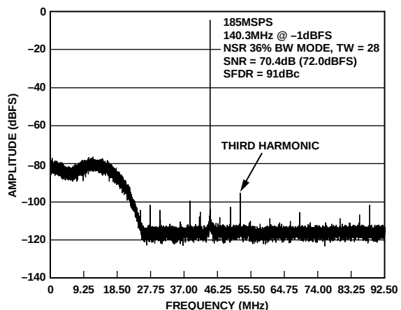
Figure 59. 36% BW Mode, Tuning Word = 28
