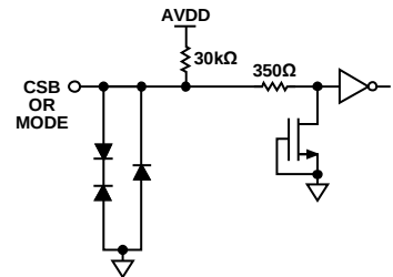
Figure 33. Equivalent CSB and MODE Input Circuit
