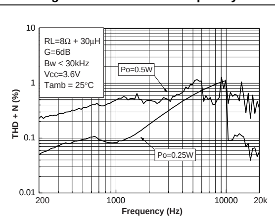
Figure 45. THD+N vs. frequency
