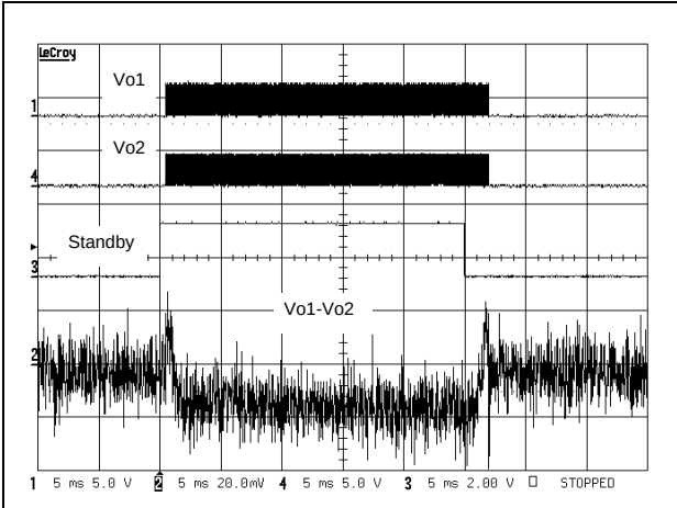
Figure 56. Startup & shutdown time V_{CC} = 3\text{ V} , G = 6\text{ dB} , C_{in} = 1\text{ }\mu\text{F} (5 ms/div)
