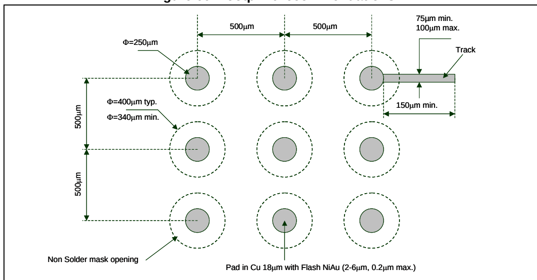
Figure 66. Footprint recommendations
