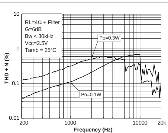
Figure 41. THD+N vs. frequency
