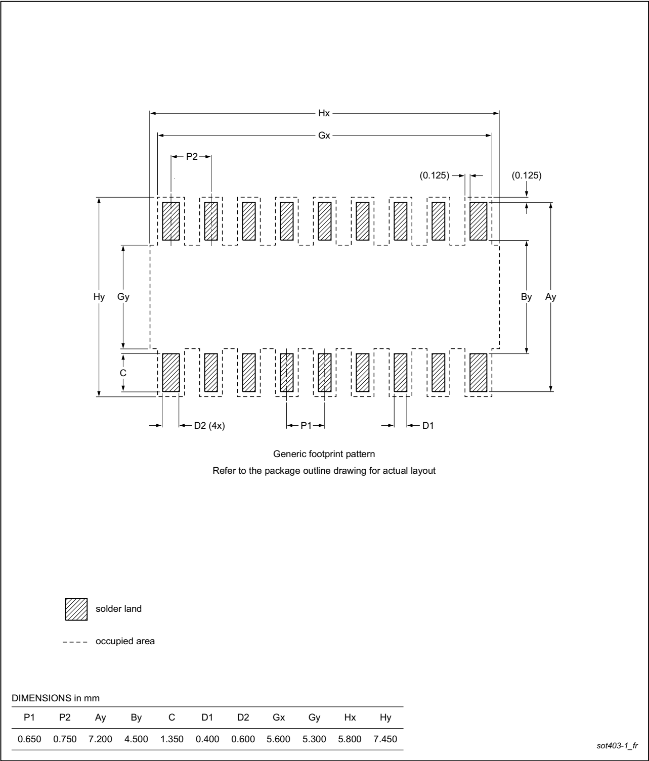
Footprint information for reflow soldering of TSSOP16 package SOT403-1
