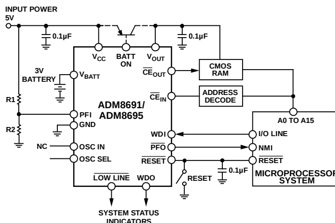
Figure 32. ADM8691/ADM8695 Typical Application
