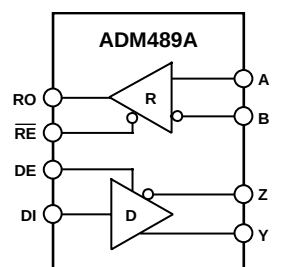
Figure 2. ADM489A
