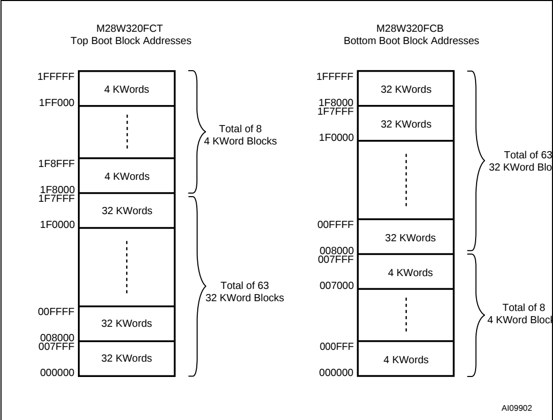
Figure 4. Block Addresses
