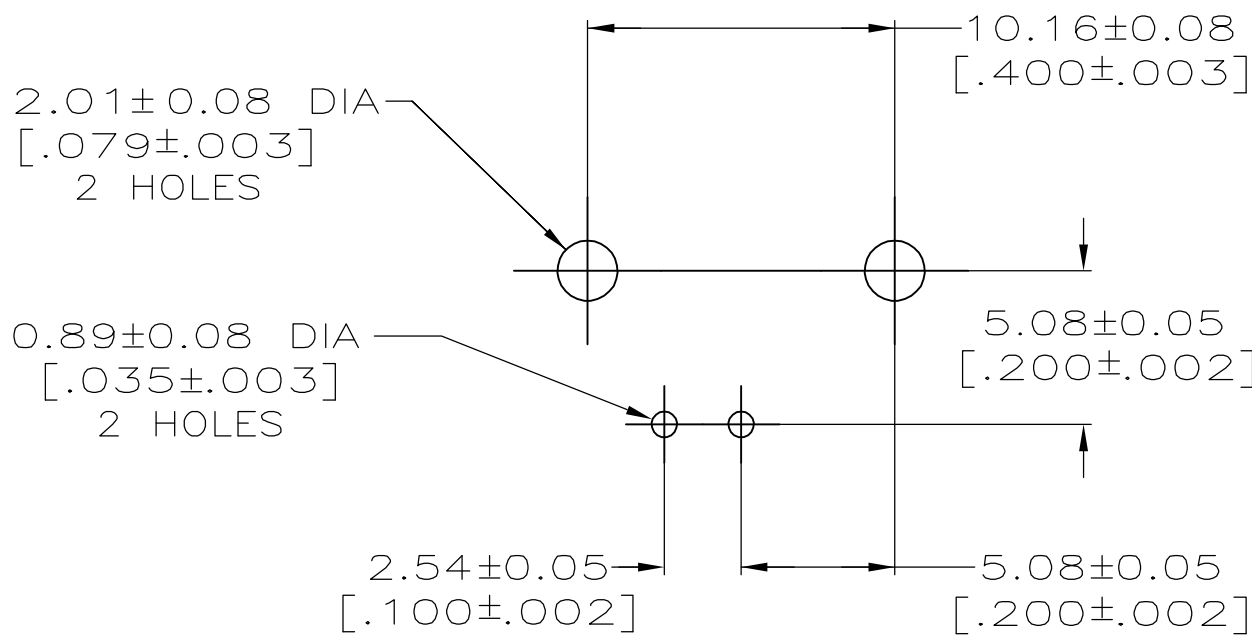
PCB CONFIGURATION
