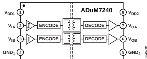
Figure 1. ADuM7240
