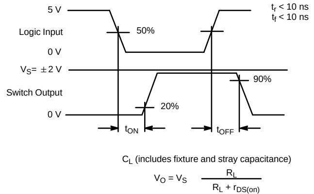
FIGURE 2. Switching Time
