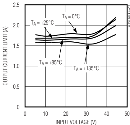
OUTPUT CURRENT LIMIT vs. INPUT VOLTAGE
