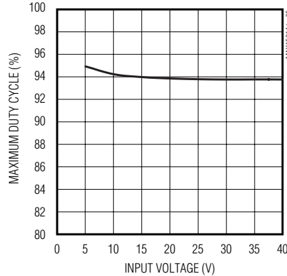
MAXIMUM DUTY CYCLE vs. INPUT VOLTAGE (MAX15015A)
