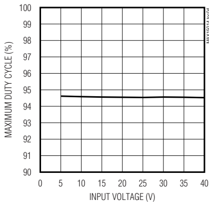
MAXIMUM DUTY CYCLE vs. INPUT VOLTAGE (MAX15016A)
