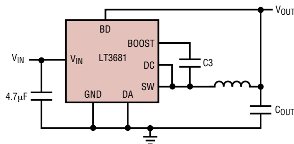
(5a) For V_{\text{OUT}} > 2.8\text{V}
