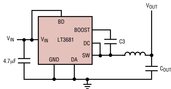
(5c) For V_{\text{OUT}} < 2.5\text{V}
