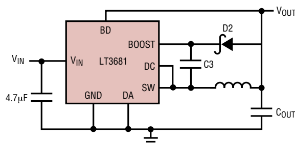
(5b) For 2.5\text{V} < V_{\text{OUT}} < 2.8\text{V}
