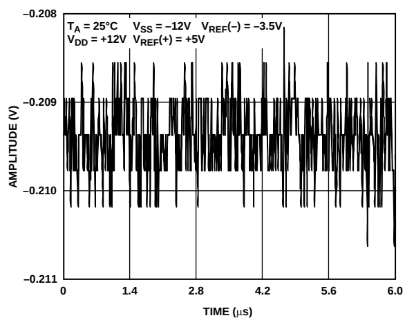
Figure 16. Digital Feedthrough
