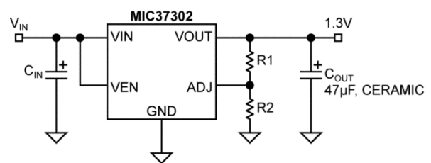
Adjustable Regulator
