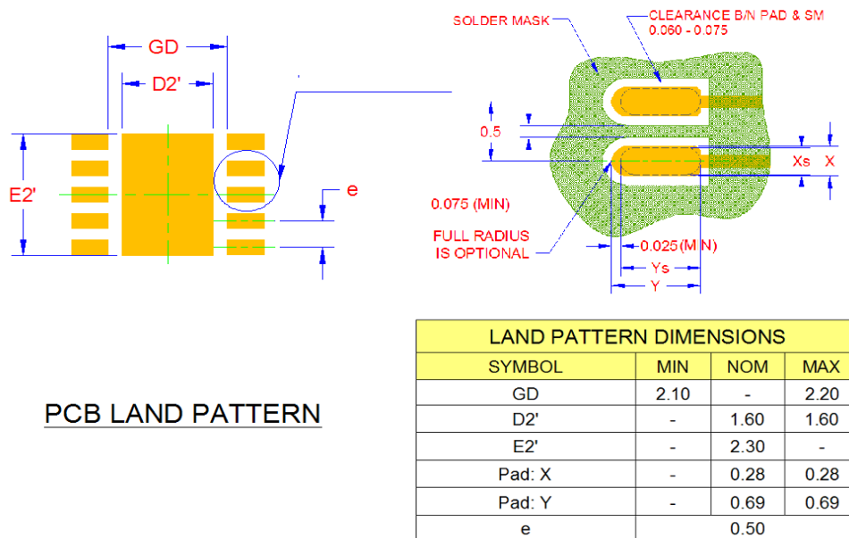
Figure 8.3 10 Pin DFN PCB Footprint
