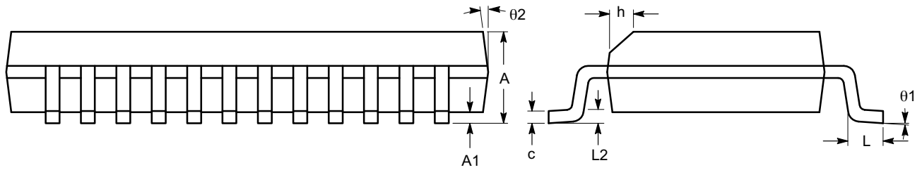
END VIEW
