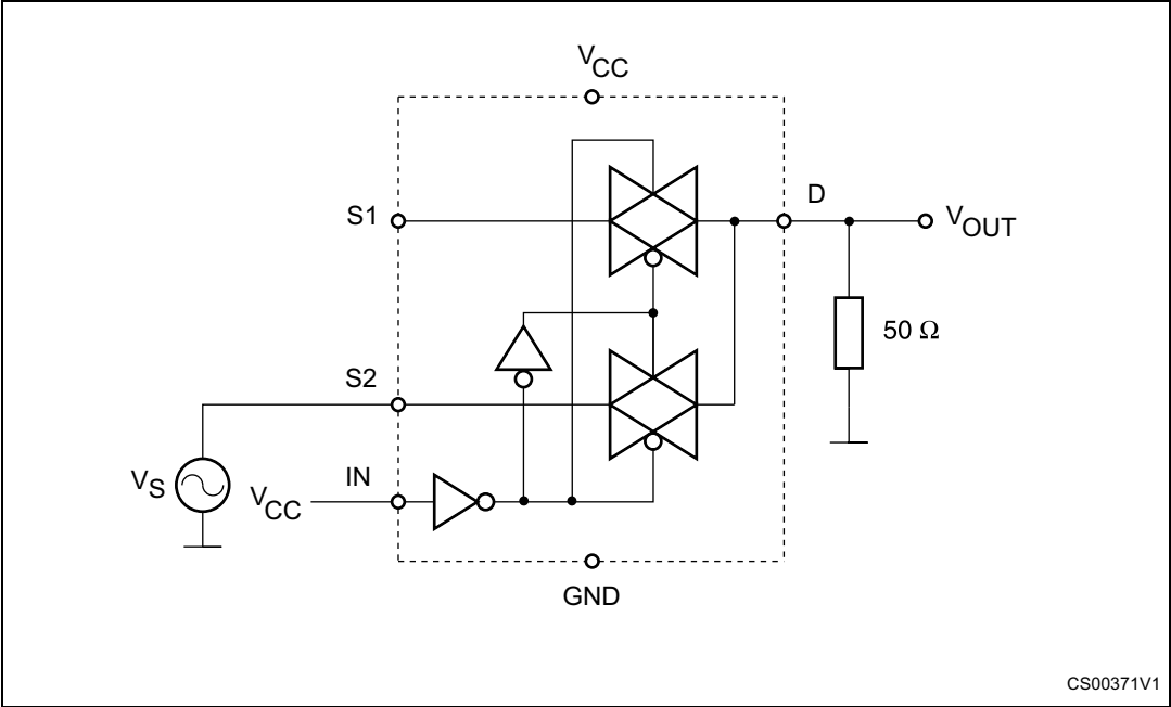
Figure 4. Bandwidth
