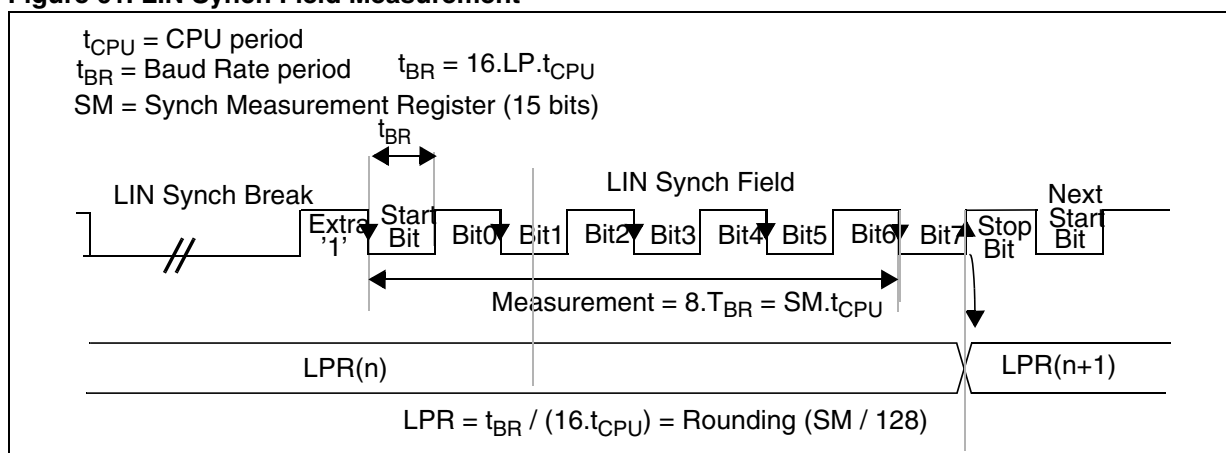
Figure 61. LIN Synch Field Measurement
