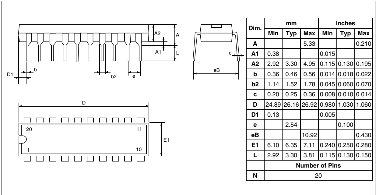
Figure 106. 20-Pin Plastic Dual In-Line Package, 300-mil Width
