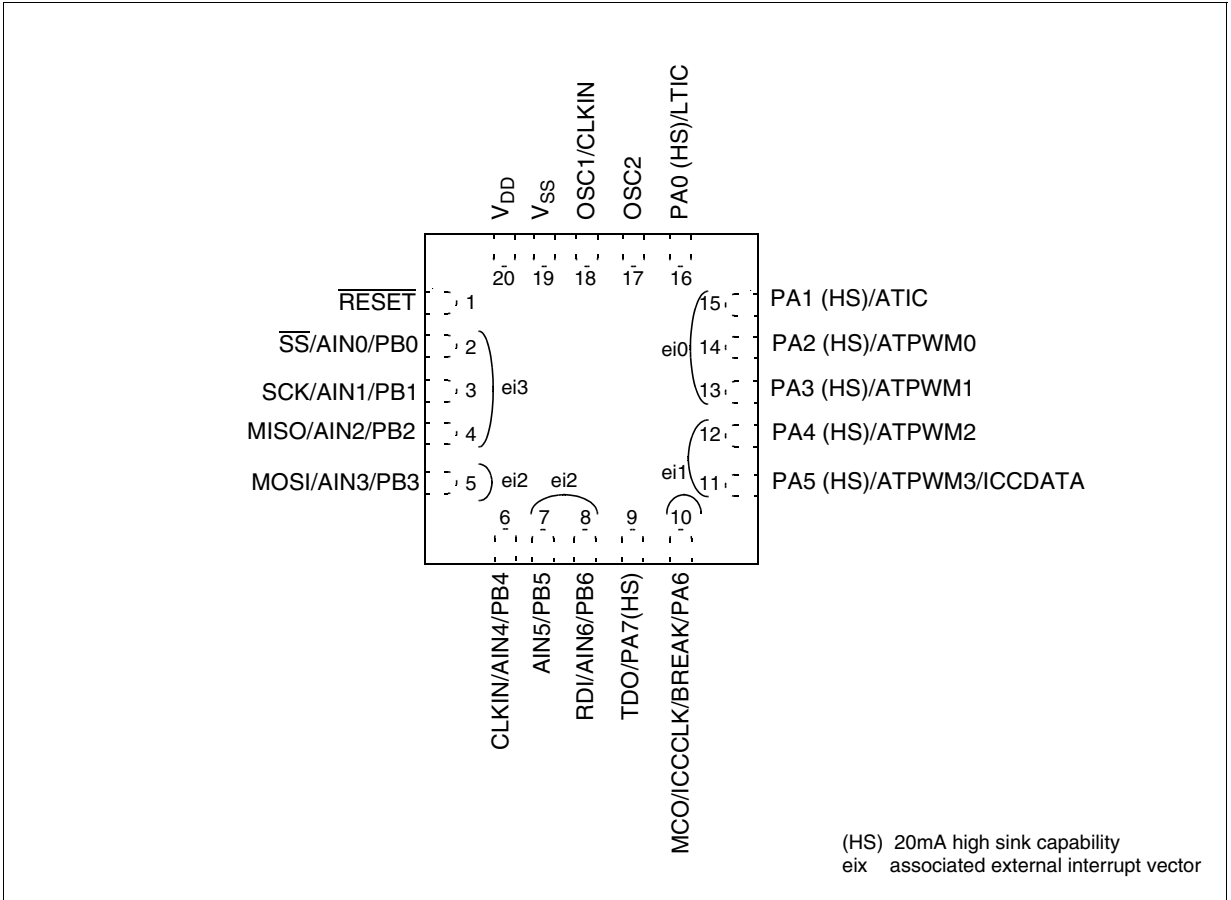
Figure 2. 20-Pin QFN Package Pinout
