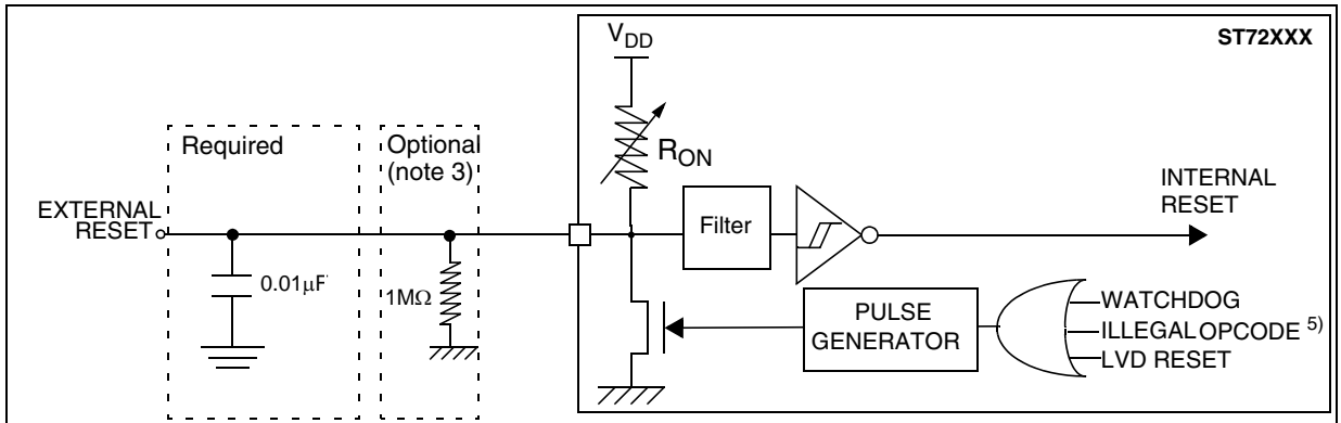
Figure 98. \overline{\text{RESET}} pin protection when LVD is disabled. 1)
