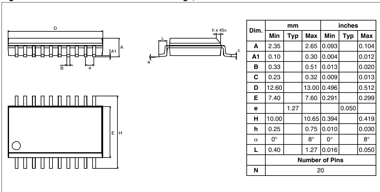
Figure 105. 20-Pin Plastic Small Outline Package, 300-mil Width
