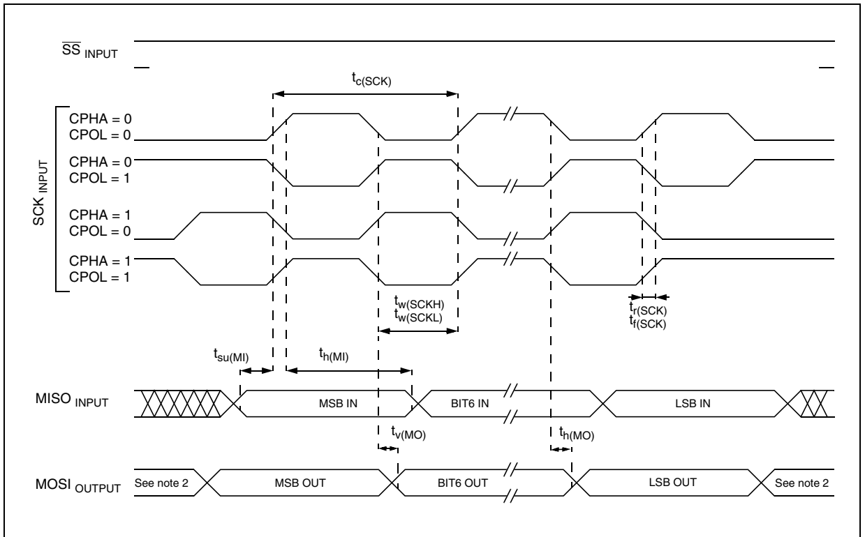
Figure 101. SPI Master Timing Diagram 1)
