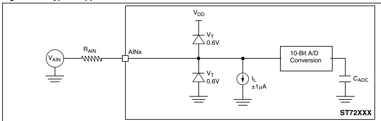
Figure 102. Typical Application with ADC
