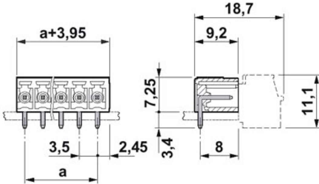
Dimensioned drawing
