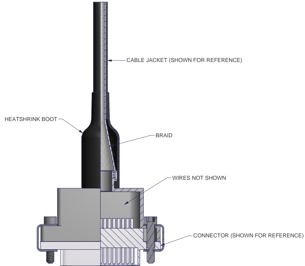
KIT ASSEMBLED WITH CONNECTOR
