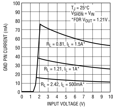
LT1963 GND Pin Current
