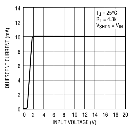
LT1963 Quiescent Current
