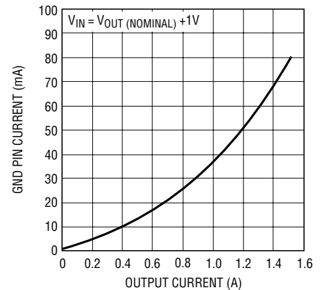
GND Pin Current vs I LOAD
