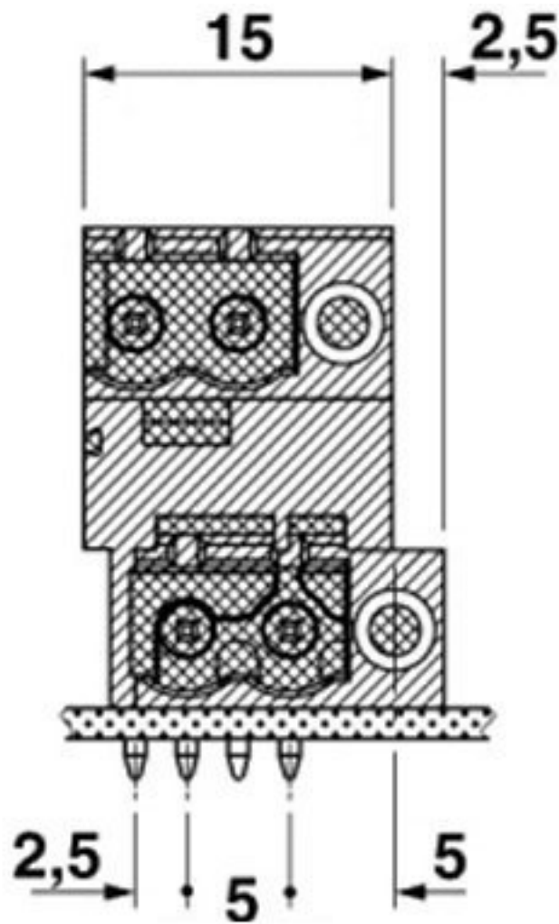
Dimensioned drawing
