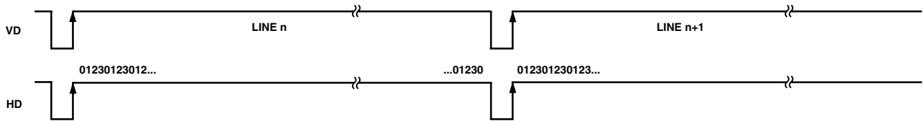
Figure 14. PxGA Mode 4 (4-Color) Frame/Line Gain Register Sequence
