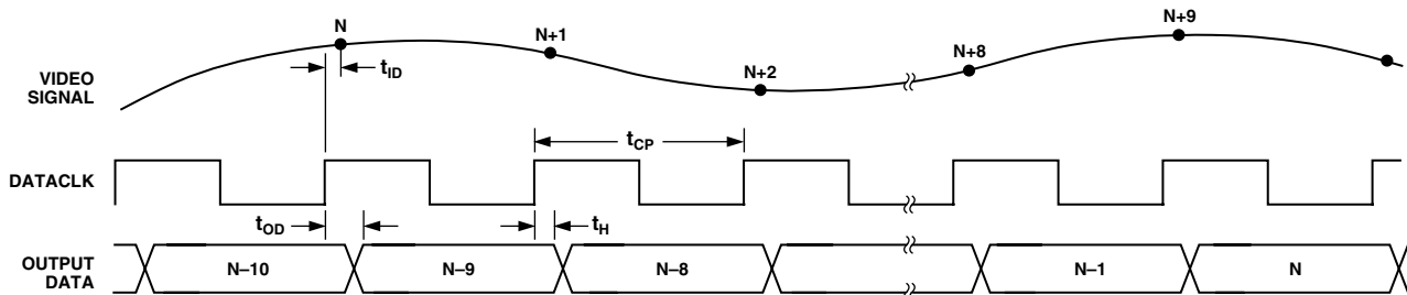
Figure 7. AUX-Mode Timing
