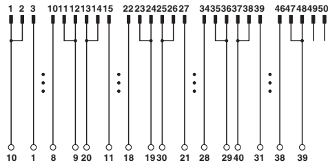
Connection scheme: FLKM 50/MODI-TSX/Q
