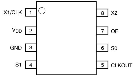
Figure 2. NB3N501 Package Pinout, 8-Pin (150 mil) SOIC
