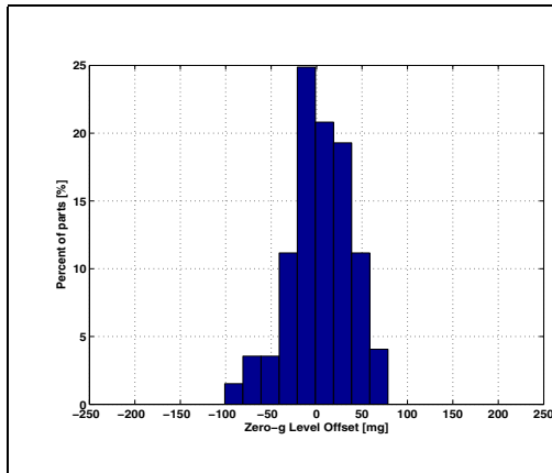
Figure 7. Y axis zero-g level at 3.3 V
