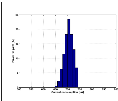
Figure 17. Current consumption in normal mode at 3.3 V
