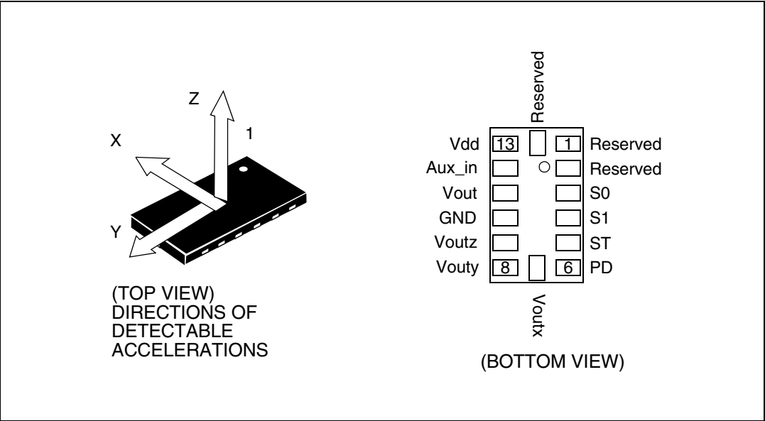
Figure 2. Pin connection
