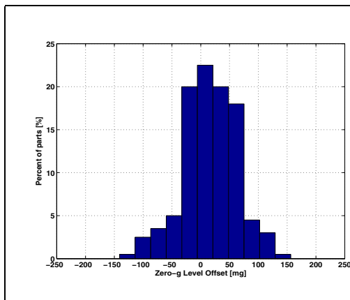
Figure 9. Z axis zero-g level at 3.3 V
