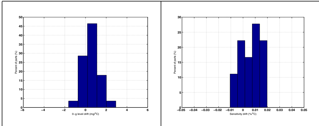
Figure 13. Y axis zero-g level change vs. temperature at 3.3 V Figure 14. Y axis sensitivity-g change vs. temperature at 3.3 V
